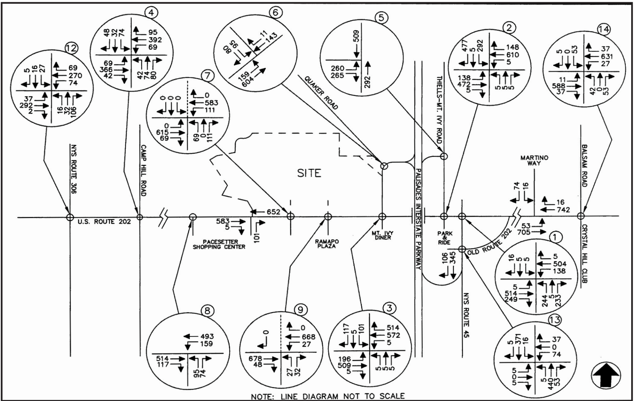
Figure 3.5-7: 2011 Projected Traffic Volumes Weekend Peak Saturday Highway Hour Minisceongo Park
